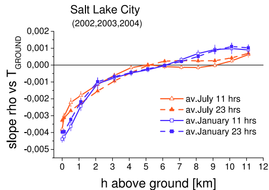
Figure 3: Slope of the correlation shown in Fig. 2 as a function of altitude, at different times of day in summer and winter at Salt Lake City.
