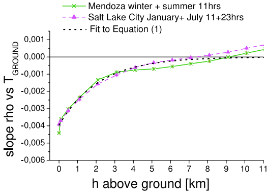
Figure 4: Comparison of the correlation slopes at Salt Lake City and Mendoza. The dotted line represents the fits of Eq.1.
