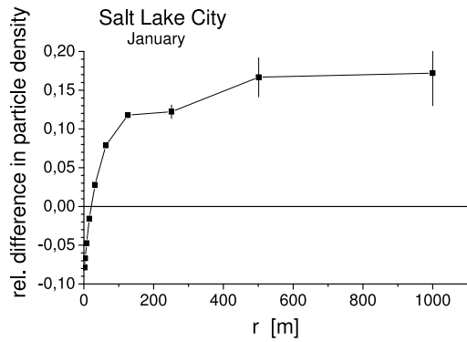
Figure 1: Relative difference in lateral distribution of particle density in a vertical 10^{19} eV proton shower simulated using atmospheric profiles in two extreme January days at Salt Lake City.
