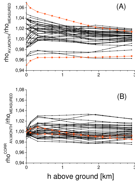
Figure 5: (A) Ratios of the average monthly profile of air density to profiles actually measured in many January days at Salt Lake City; (B) Ratios of the corrected average profile to daily measurements.
