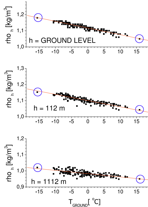
Figure 2: Example of correlation of air density at two different altitudes above ground, with temperature at the ground level. The circles mark the extremely warm and cold days used to prepare Fig. 1.
