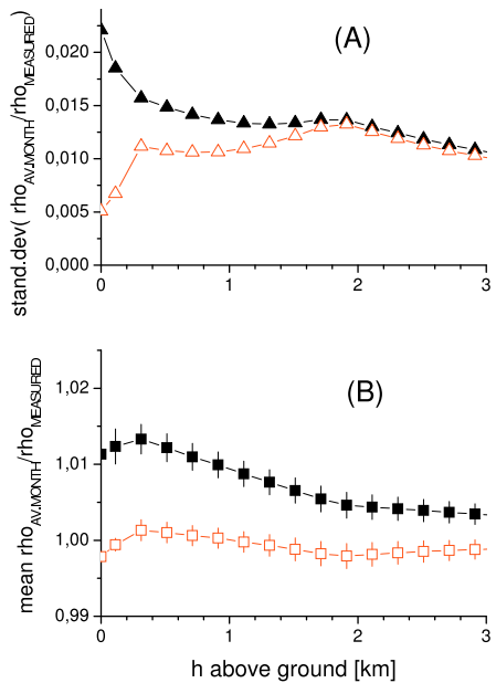
Figure 6: (A) Standard deviation and (B) mean of ratios shown in Fig.5 as a function of altitude. The filled symbols pertain to uncorrected density profiles of Fig.5A, while the open symbols concern the corrected profiles of Fig.5B.
