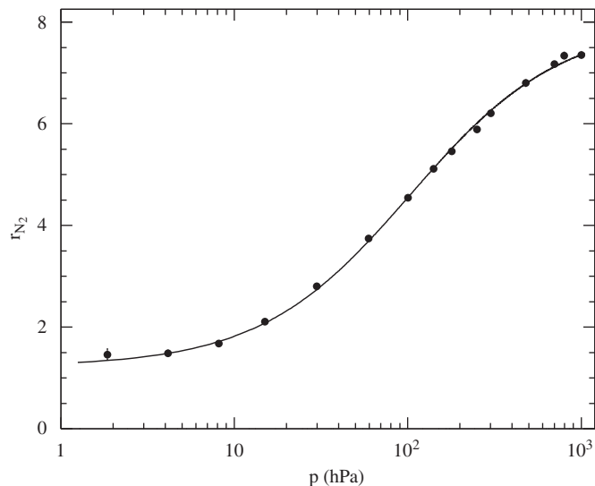
Fig. 3. Ratio of nitrogen to air signals as a function of pressure, together with the fit used to measure p'_{air} of the 337.1 nm band.
