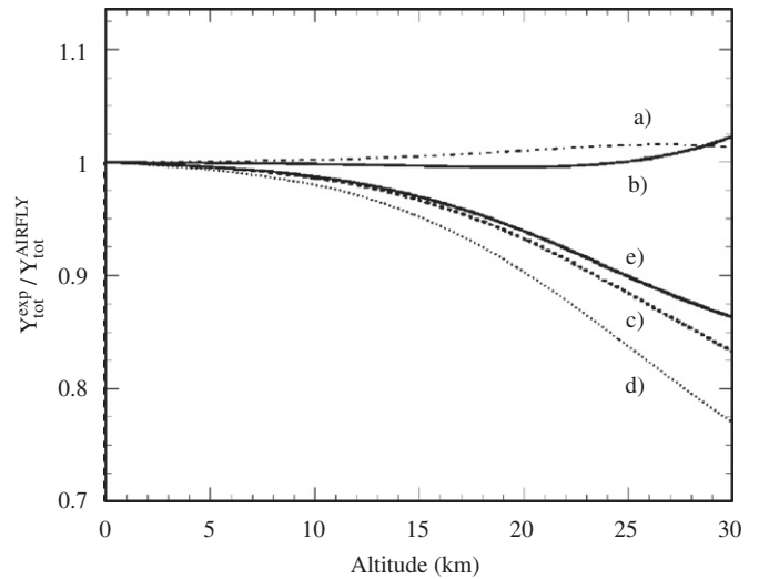
Fig. 5. Ratio of the total fluorescence yield in the range 300–400 nm as measured by other experiments to the one measured by AIRFLY as a function of altitude: (a) Belz et al., (b) Bunner, (c) Nagano et al., (d) Kakimoto et al., (e) Colin et al.
