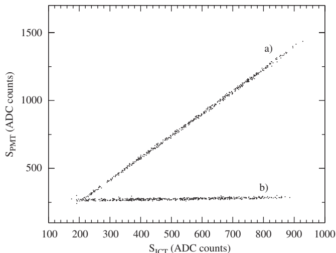
Fig. 2. Correlation of PMT and ICT signals for a fluorescence run (a) and a background run (b) in nitrogen at 180 hPa.
