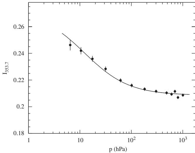
Fig. 4. Relative intensity I_{353.7} of the 2P(1,2)-transition as a function of pressure. The full line represents the best fit to p'_{\text{air}}(353.7) .
