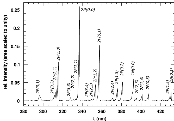
Fig. 1. Air fluorescence spectrum excited by 3 MeV electrons at 800 hPa. Labels indicate 21 major transitions.
